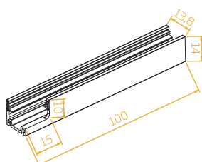
Cable-exit Mounting Clip-Side
